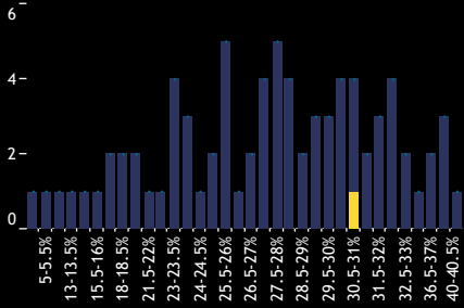
1. Histogram of Fund Weights As of 2/28/2025
